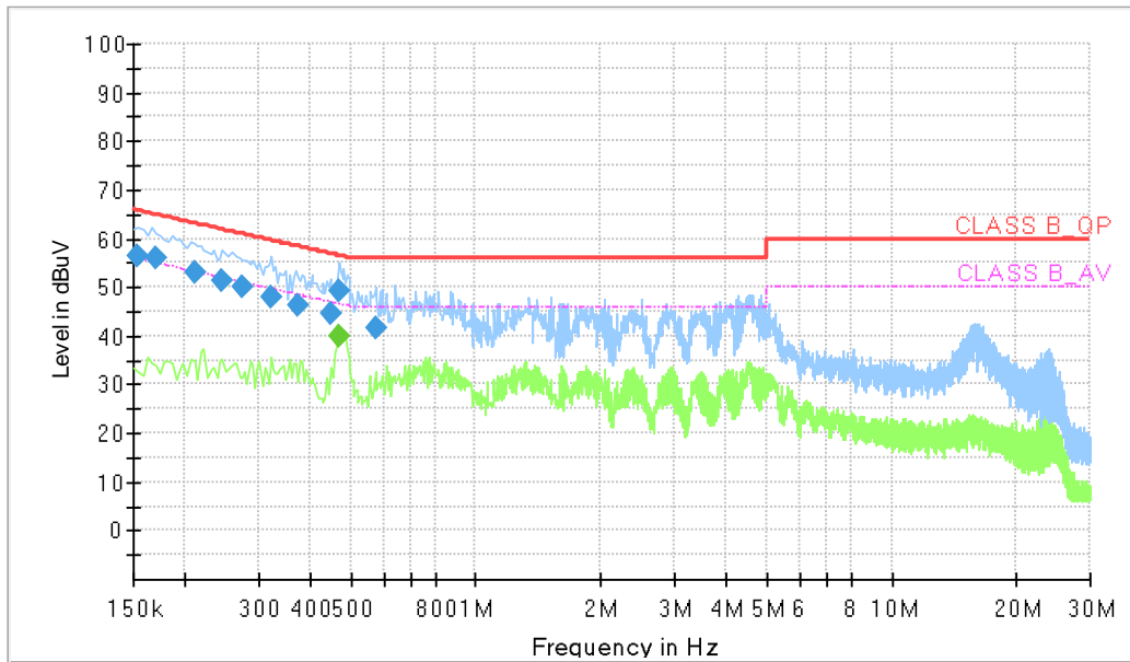
— Preview Result 2-AVG — Preview Result 1-PK+ — CLASS B_QP - - - CLASS B_AV ◆ Fina_Result QPK ◆ Fina_Result CAV
