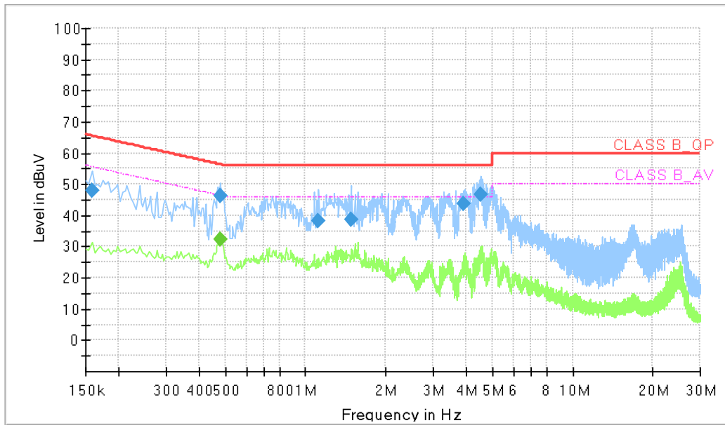
— Preview Result 2-AVG — Preview Result 1-PK+ — CLASS B_QP - - - CLASS B_AV ◆ Final_Result QPK ◆ Final_Result CAV
